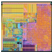
Alien Higgs 10
